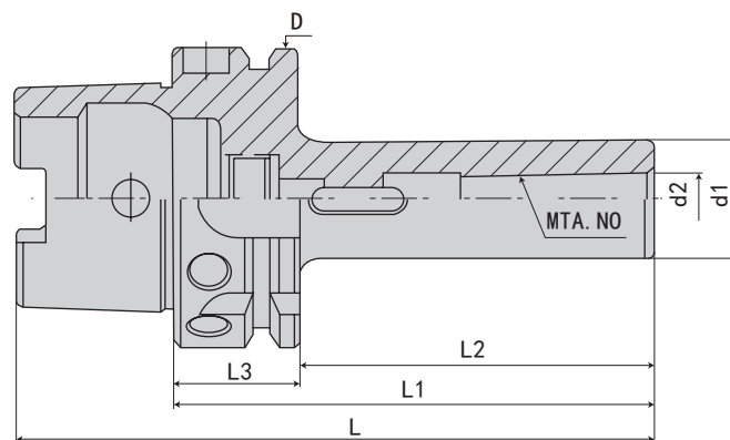
HSK63A-MTA TAPER ADAPTER(MORSE)
