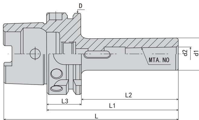
HSK50A-MTA TAPER ADAPTER(MORSE)
